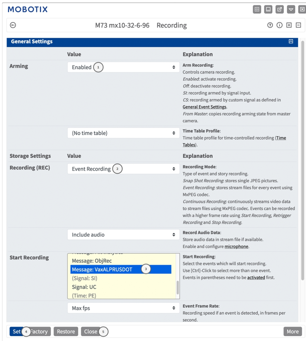
Fig. 24: Configuration of camera recording settings
