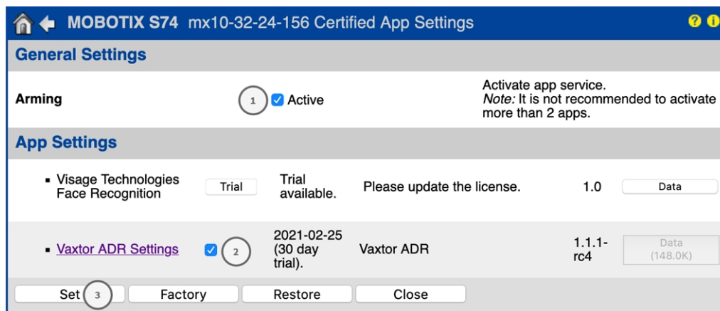
Fig. 12: Activation of Certified Apps
