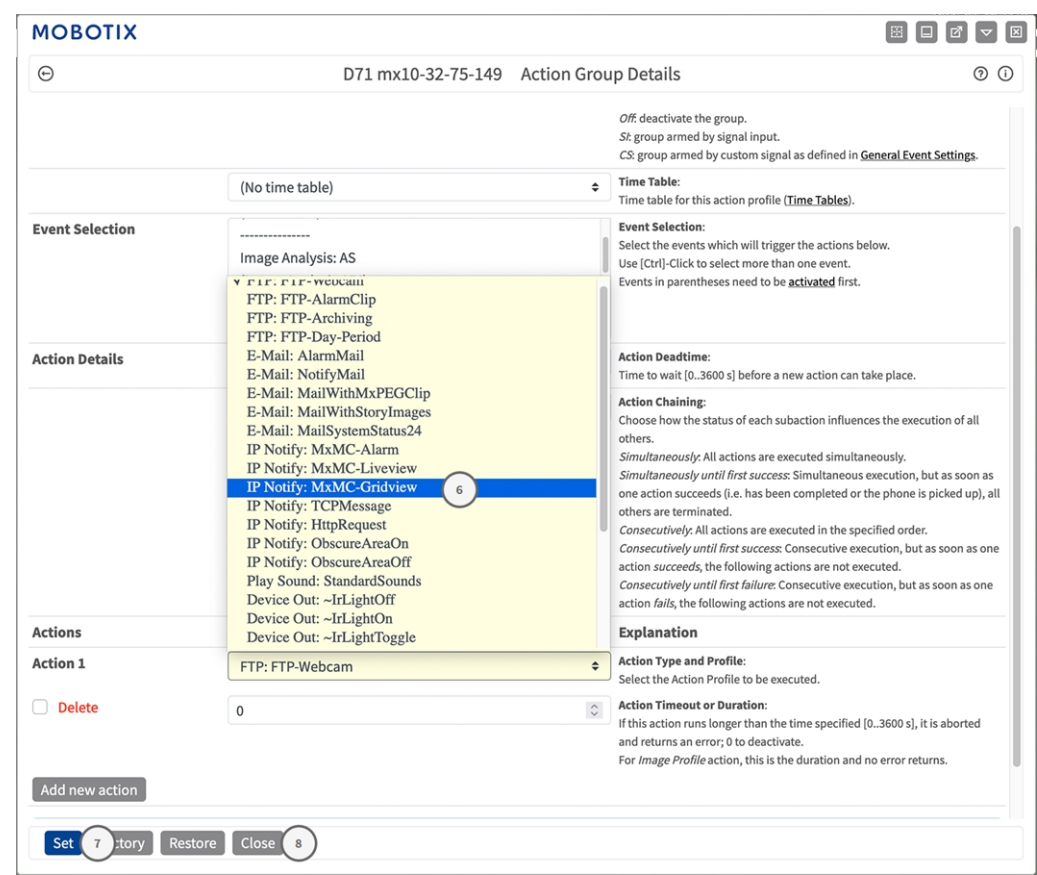
Fig. 24: Select Action Type- and Profile
