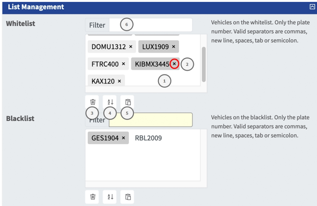
Fig. 13: Black and white lists
