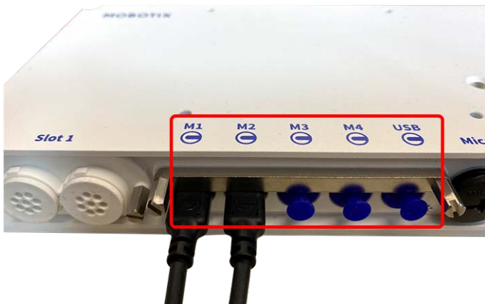
Fig. 4: 4 Module Connector Ports and 1 USB-C interface
