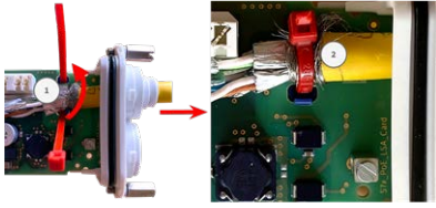
Fig. 11: Cable tie inserted beneath network cable
