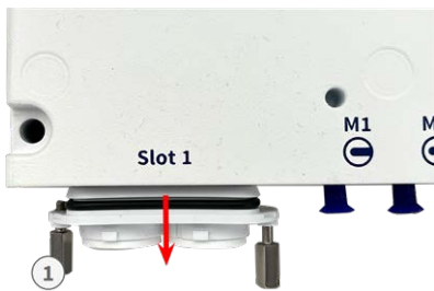
Fig. 18: Remove cover from interface board slot
