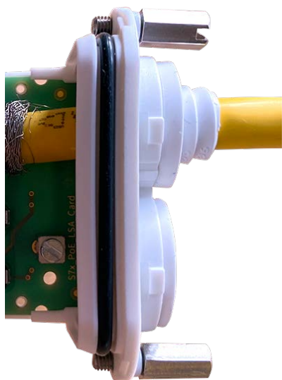
Fig. 10: Network cable inserted, plug properly seated
