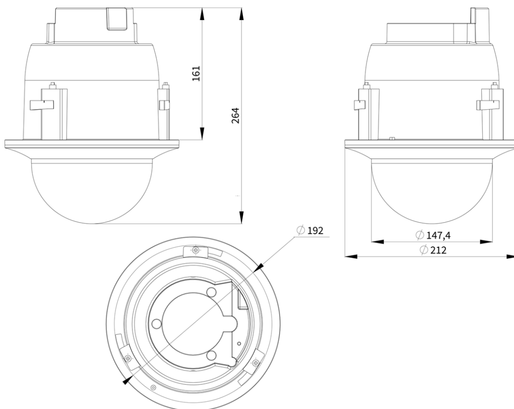
Fig. 1: 2MP Low-Light Flush-Mount Video Analytics Speed Dome: Tutte le misurazioni in mm
