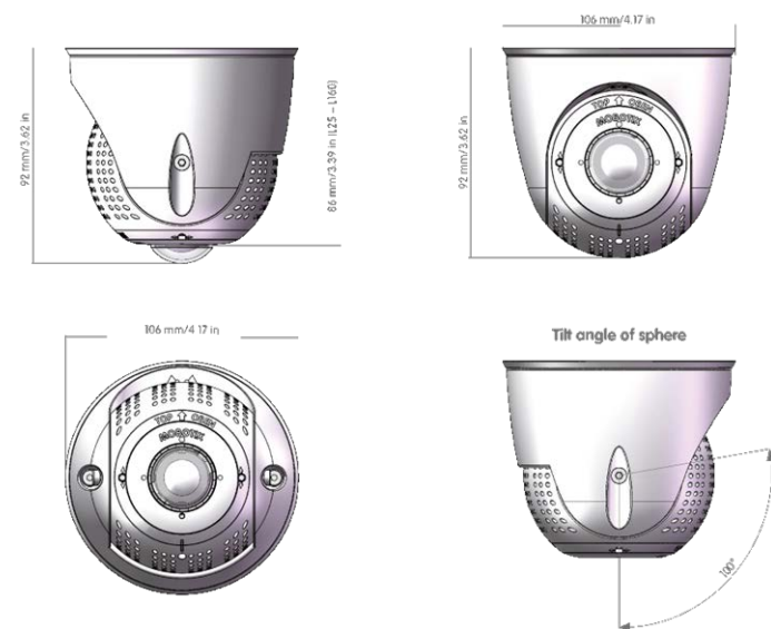
Fig. 2: PTMount
