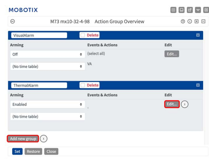
Fig. 6: Defining Action Groups
