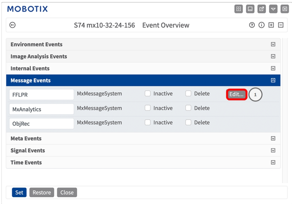
Fig. 19: Example: Generic message event from FF Group License Plate Recognition App - Region EUCA
