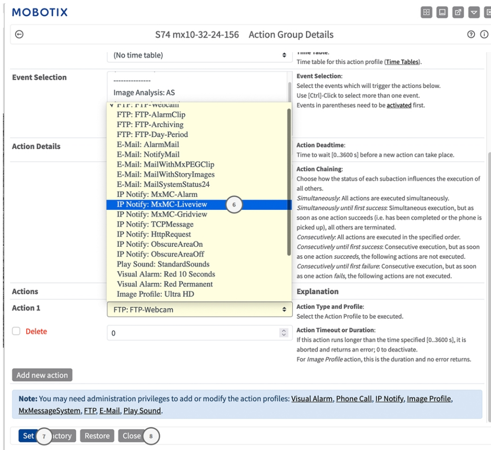
Fig. 23: Select Action Type- and Profile
