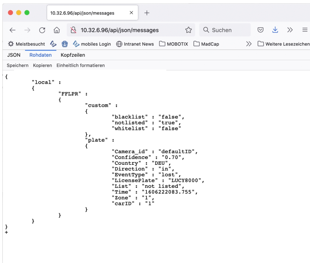
Fig. 25: Example: Meta data transmitted within a MxMessage of the FF Group License Plate Recognition App - Region EUCA
