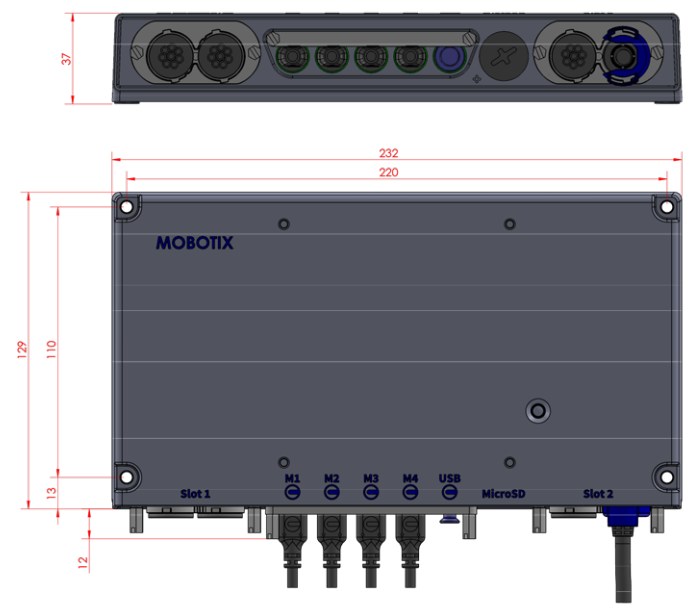
Fig. 1: MOBOTIX S74: All measurements in mm
