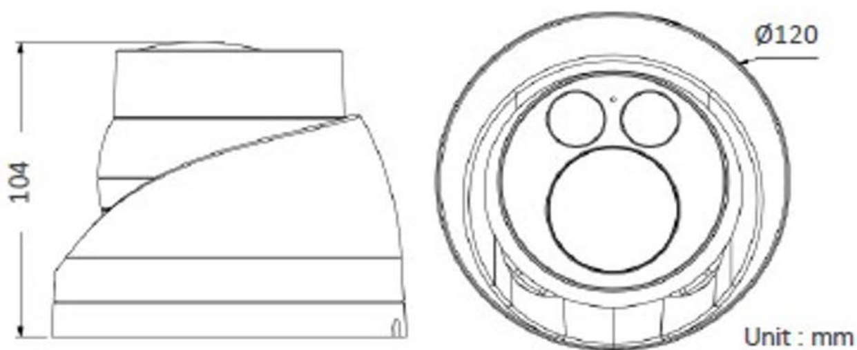
Fig. 1: Mx-VT1A-203-IR: All measurements in mm
