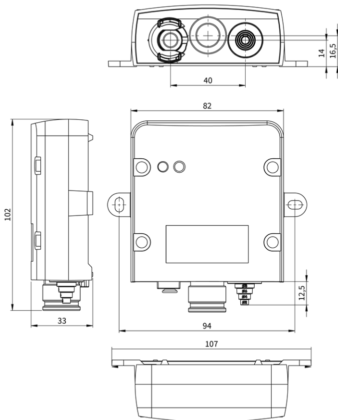
Fig. 2: MOBOTIX M73: All measurements in mm
