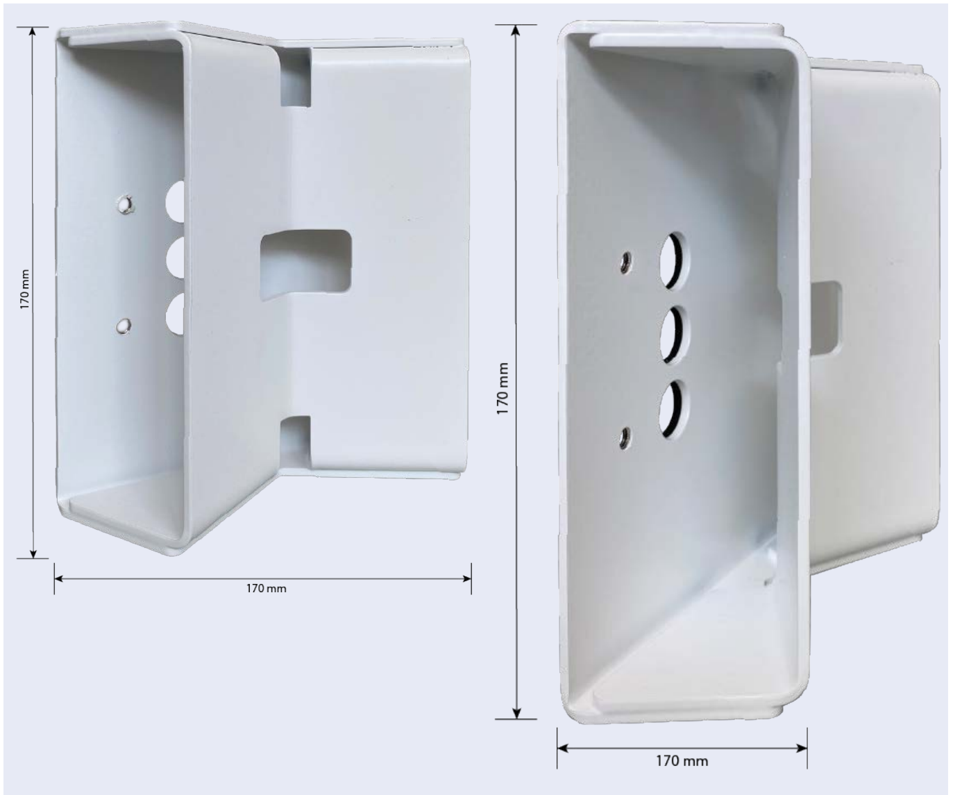
Fig. 13: Dimensions M73 pole mount – rear view
