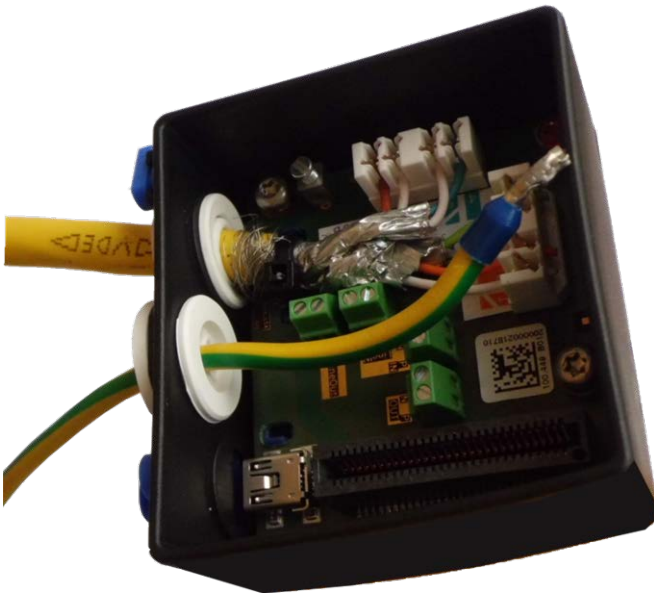
Fig. 29: Ground wire inserted, plug properly seated
