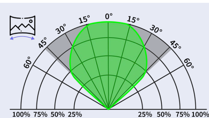
Lens With 95° Horizontal Viewing Angle
