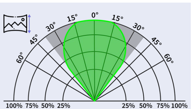
Lens With 76° Vertical Viewing Angle
