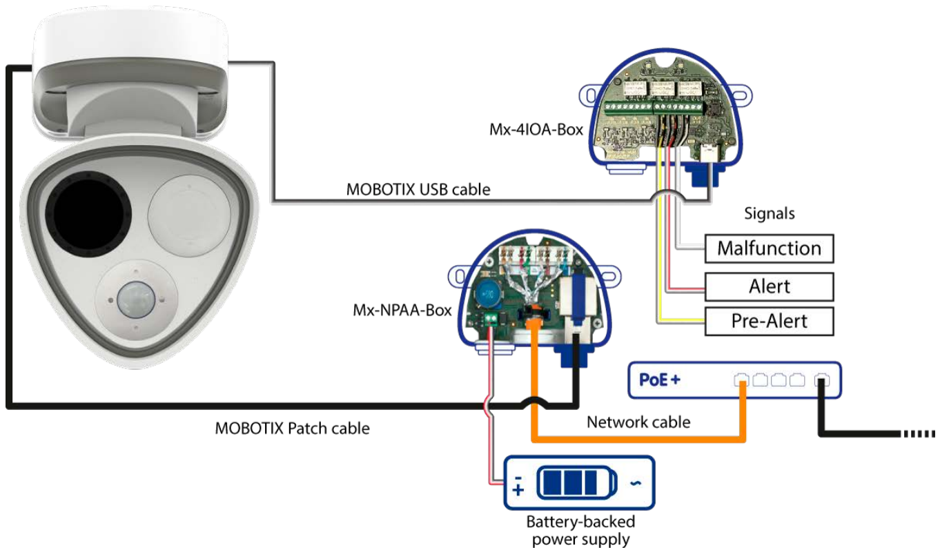
Fig. 2: Wiring of the M73 EN54 Bundle-V3
