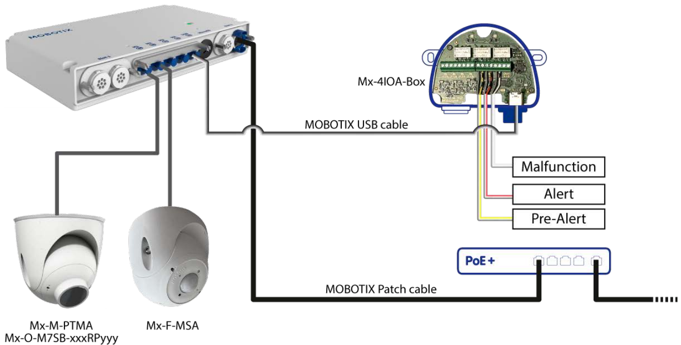
Fig. 1: Wiring of the S74 EN54 Bundle-V2
