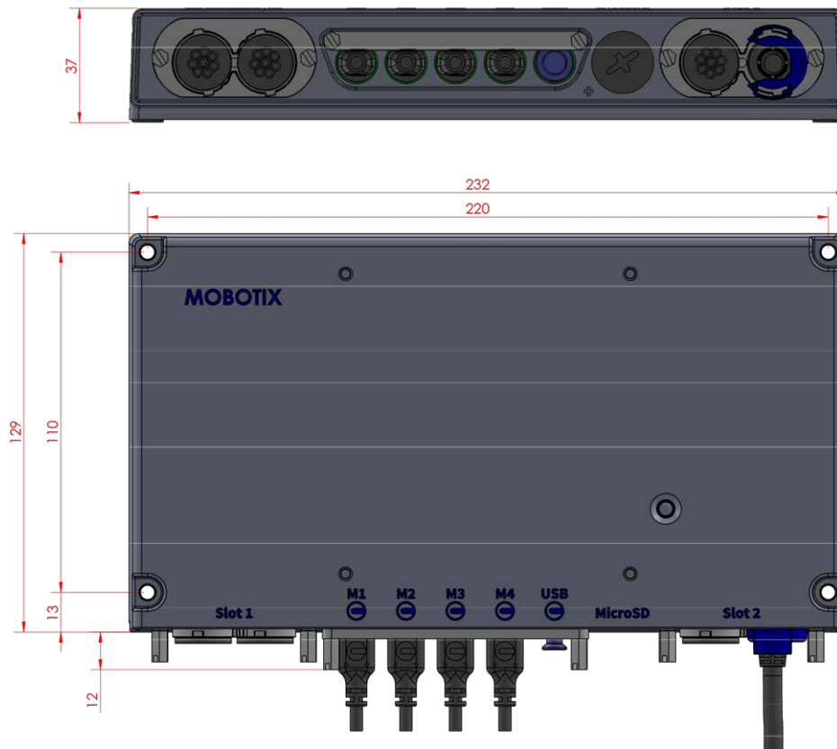
Fig. 9: MOBOTIX M73: All measurements in mm
