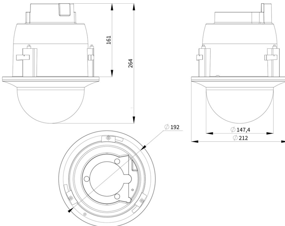
Fig. 1: Mx-SD2A-230-LL-FM-VA: All measurements in mm
