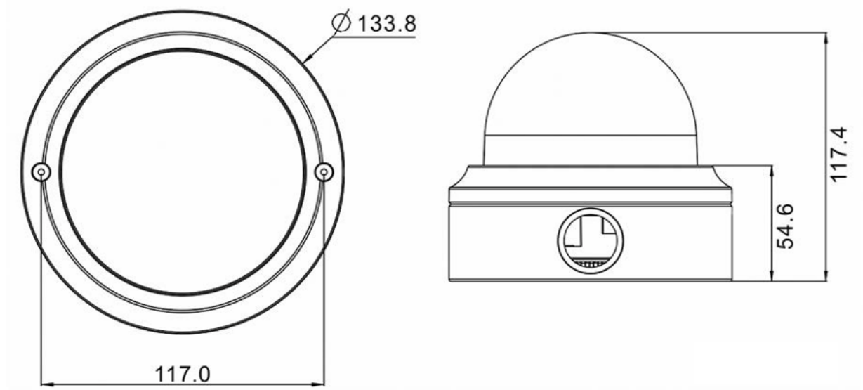
Fig. 1: Mx-VD2A-2-IR: All measurements in mm
