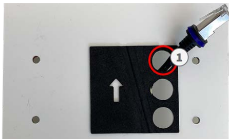
Fig. 10: Prepared for Connector Box RJ45
