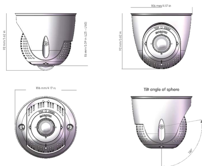
Abb. 2: PTMount
