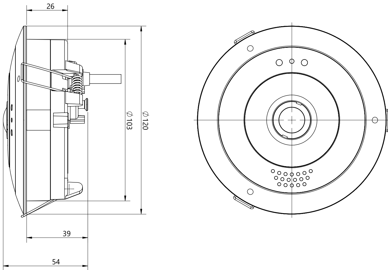
Abb. 1: MOBOTIX c ONE Nurse Assist: Alle Abmessungen in mm
